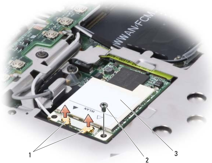
1 antenna cable connectors 2 screw 3 WLAN card
